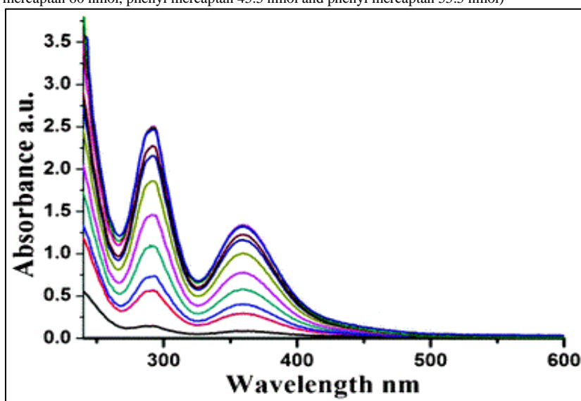
Figure-4. Absorption spectrum of CdO nanoparticles with various aryl mercaptanes during 90 (s) (concentration of CdNPs is equal to 250 ppm and 2.5 ml used, phenyl mercaptan 60 nmol, phenyl mercaptan 45.5 nmol and phenyl mercaptan 55.5 nmol)
