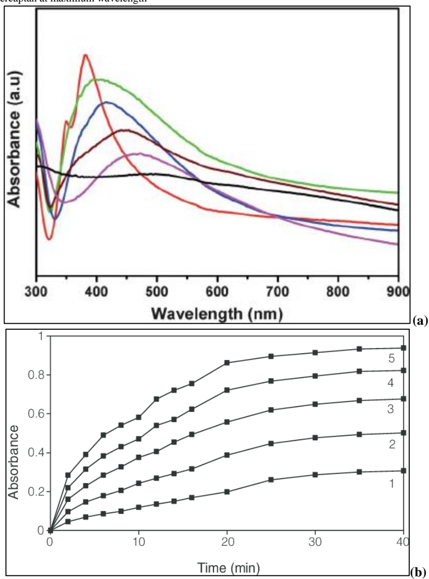
Figure-3. (a) Absorption spectrum of CdO nanoparticles–propyl mercaptan during 0–1200 (s). (b) Absorption curve against time for CdO nanoparticles–propyl mercaptan at maximum wavelength
