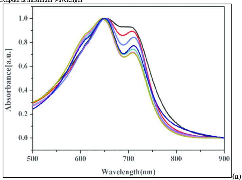
Figure-3. (a) Absorption spectrum of CdO nanoparticles–propyl mercaptan during 0–1200 (s). (b) Absorption curve against time for CdO nanoparticles–propyl mercaptan at maximum wavelength
