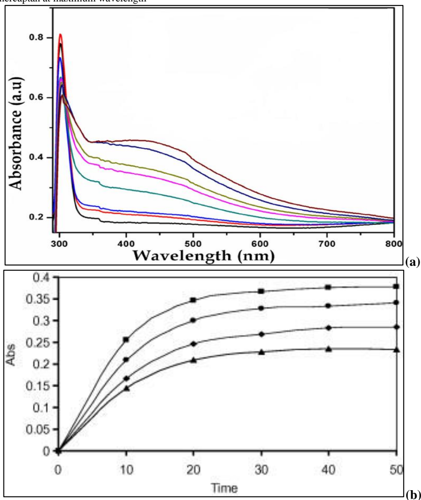
Figure-1. (a) Absorption spectrum of CdO nanoparticles–phenyl mercaptan during 0–1200 (s). (b) Absorption curve against time for CdO nanoparticles–phenyl mercaptan at maximum wavelength
